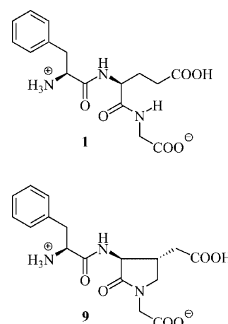
Scheme 2. Structures of FEG ( 1 ) and of its constrained analogue 9 .
