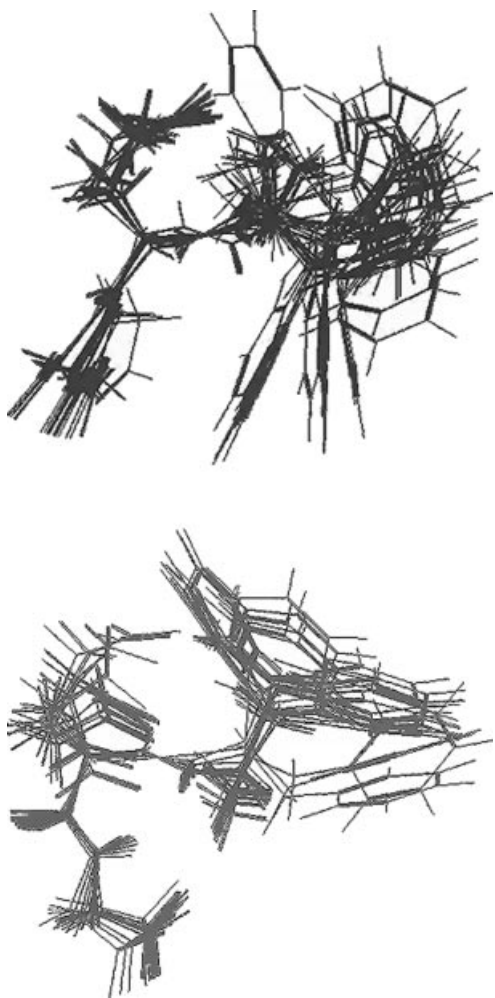
Figure 1. Cluster analysis of FEG ( 1 ). Cluster no. 1 (top) and no. 2 (bottom), with a cluster value of 0.4 for superimposing \phi_2 and \psi_2 .
