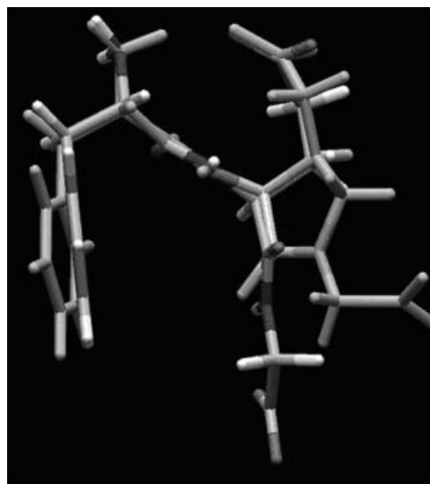
Figure 3. Superimposition of the FEG lowest-energy conformer and the most representative structure in cluster no. 2 of analogue 9 .
