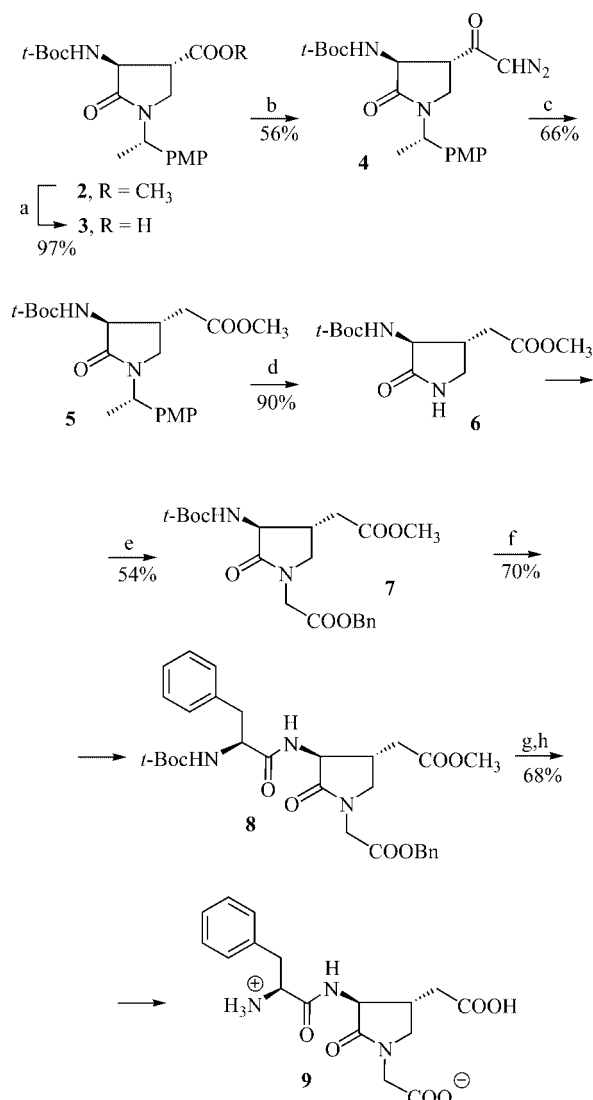
Scheme 1. (a) 1 M NaOH, then 1 M HCl; (b) ClCOOCH 3 , Et 3 N, DCM, 0 °C, then CH 2 N 2 , -10 °C; (c) PhCOOAg, Et 3 N, MeOH, 0 °C; (d) CAN, CH 3 CN/H 2 O, room temp.; (e) NaH, THF, 0 °C, then BrCH 2 COOBn, THF, 0 °C to room temp.; (f) TFA, DCM, room temp., then Et 3 N, t Boc-Phe, EDCl, DCM, room temp.; (g) 2 M NaOH, followed by 1 M HCl; (h) TFA, then Dowex 50, 1 M NH 4 OH.
