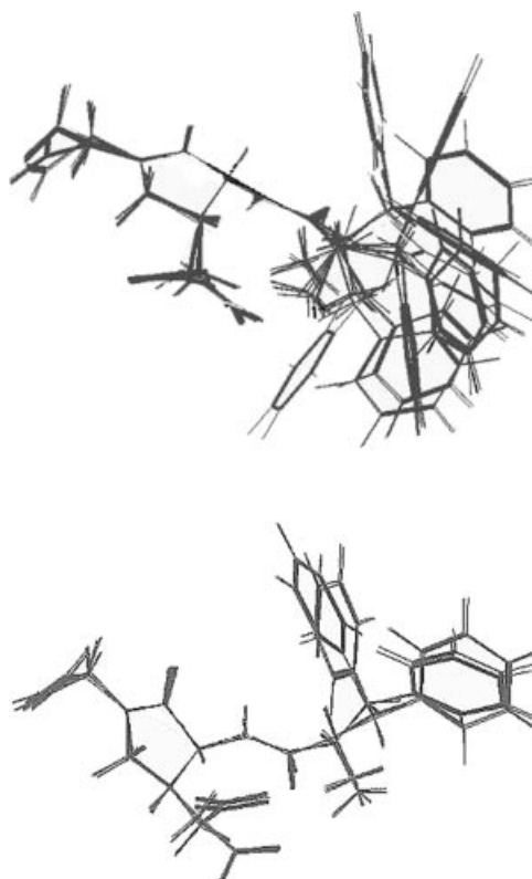
Figure 2. Cluster analysis of mimetic 9 . Cluster no. 1 (top) and no. 2 (bottom), with a cluster value of 0.2 for superimposing \phi_2 and \psi_2 .
